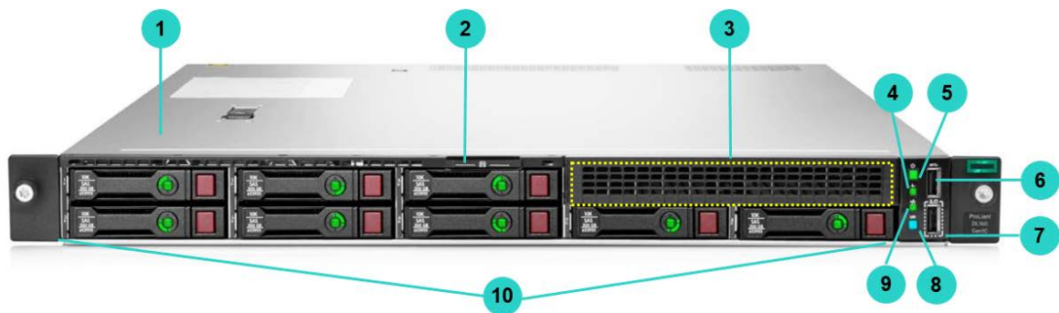
8 SFF chassis - Front View
