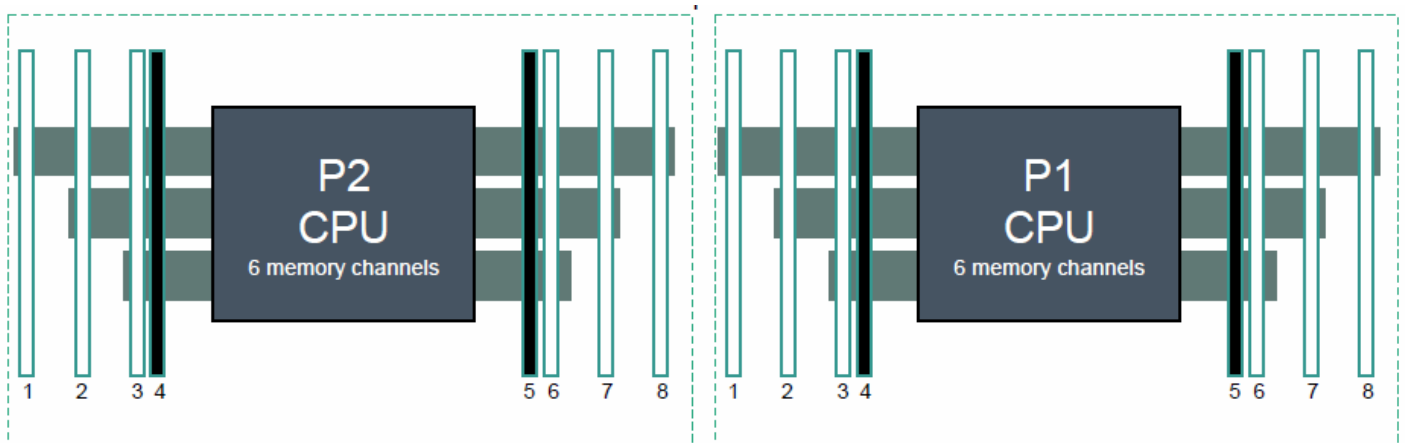
HPE DL160/DL180 Gen 10 Servers Front Server
